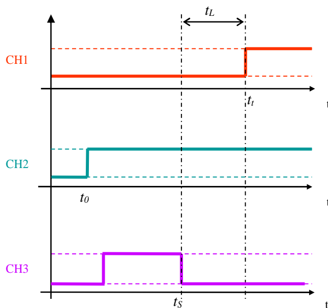
Figure 10: Minimum listen time after detection, t_L , measurement
