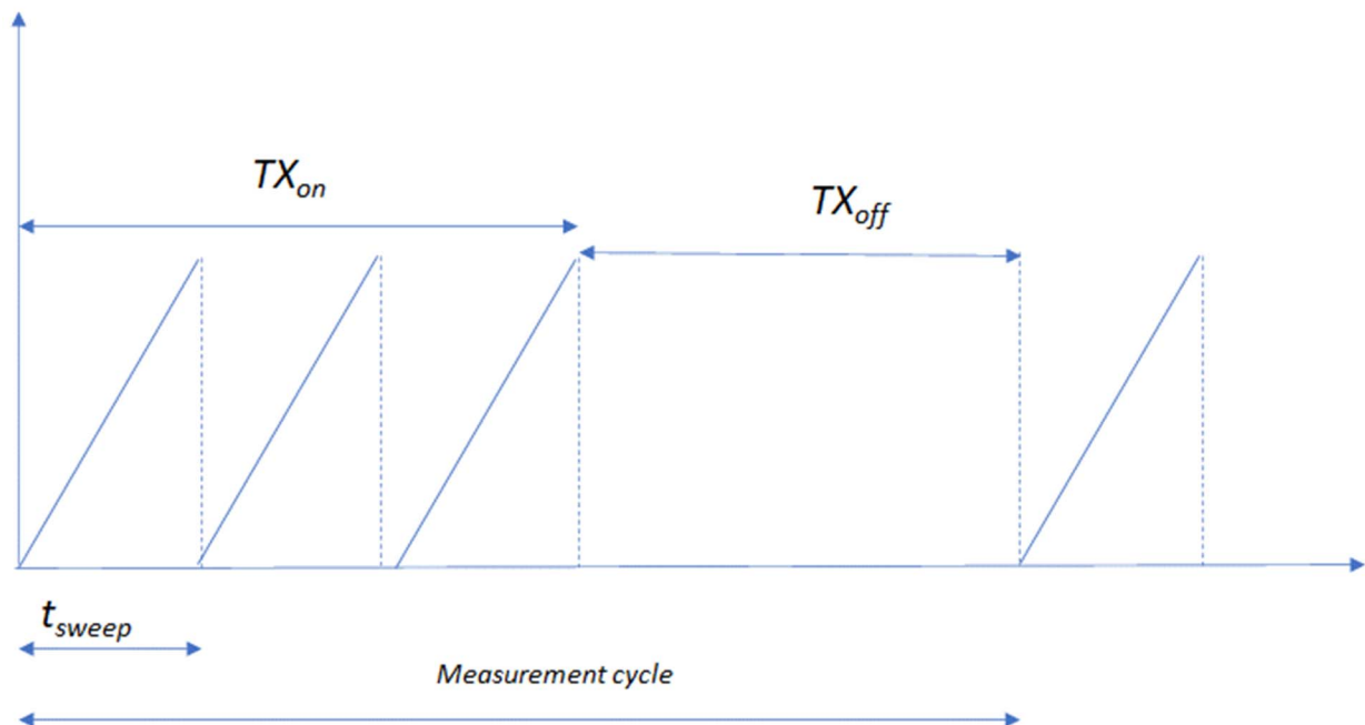
Figure E.1: Example of an automotive radar signal
