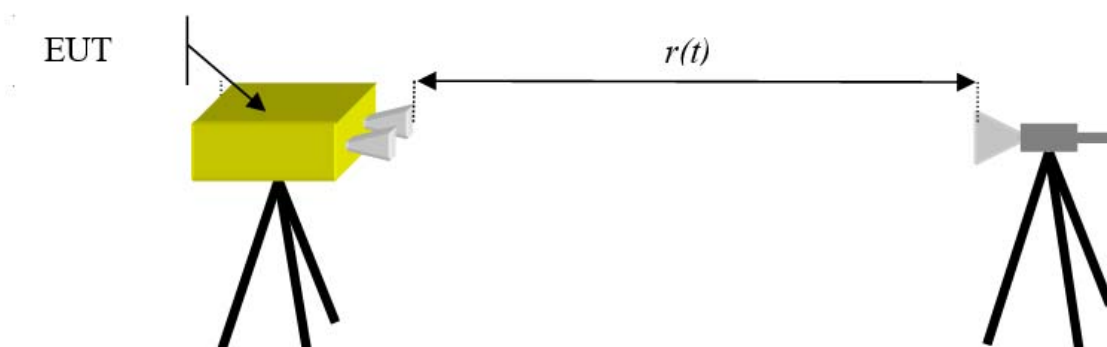
Figure 7: Setup for RBS measurement
