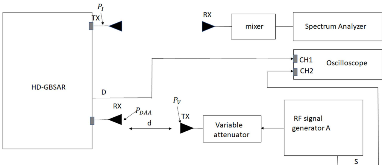
Figure 12: DAA measurement arrangement
