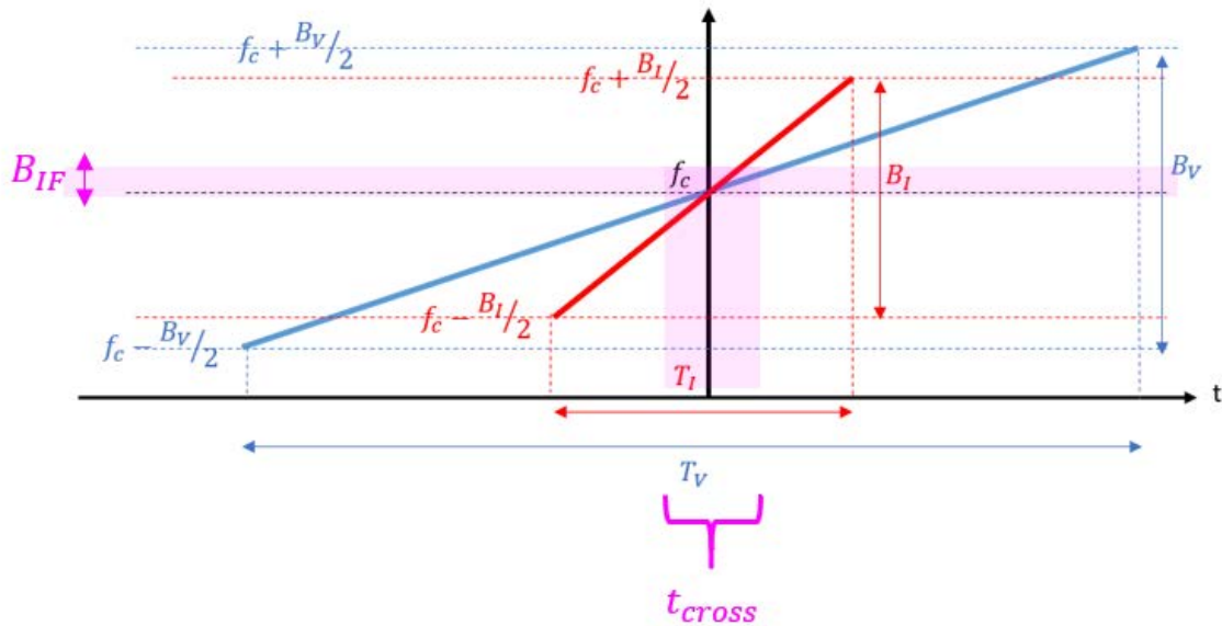
Figure E.2: Crossing time t_{cross} between interfering signals
