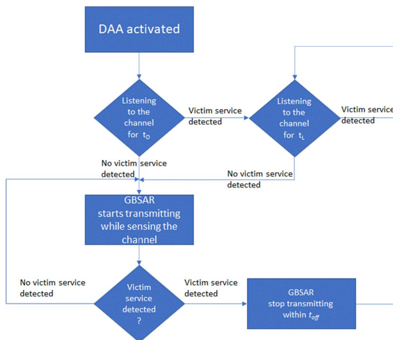
Figure 3: GBSAR Detect and Avoid overview
