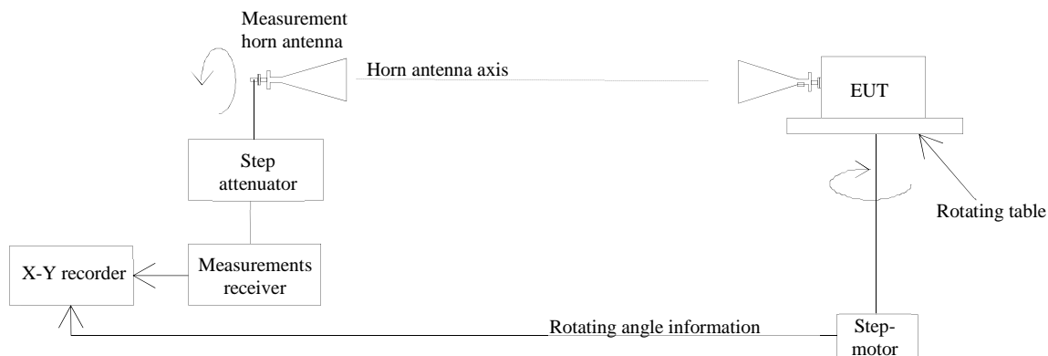
Figure 13: Test setup for measurement of antenna pattern
