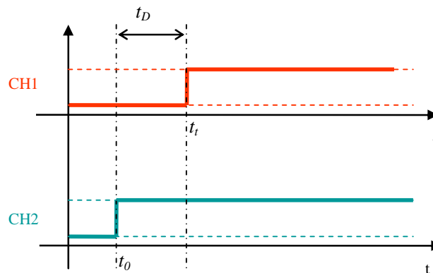
Figure 9: Minimum listen time, t_D , measurement
