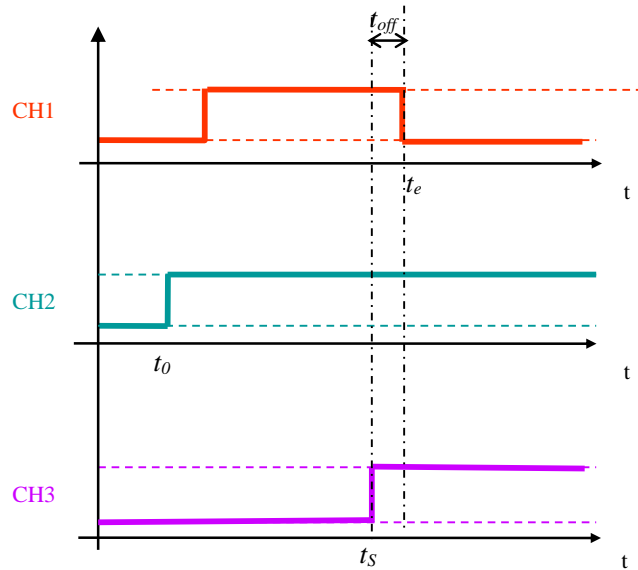
Figure 11: Maximum transmit switch-off time, t_{off} , measurement
