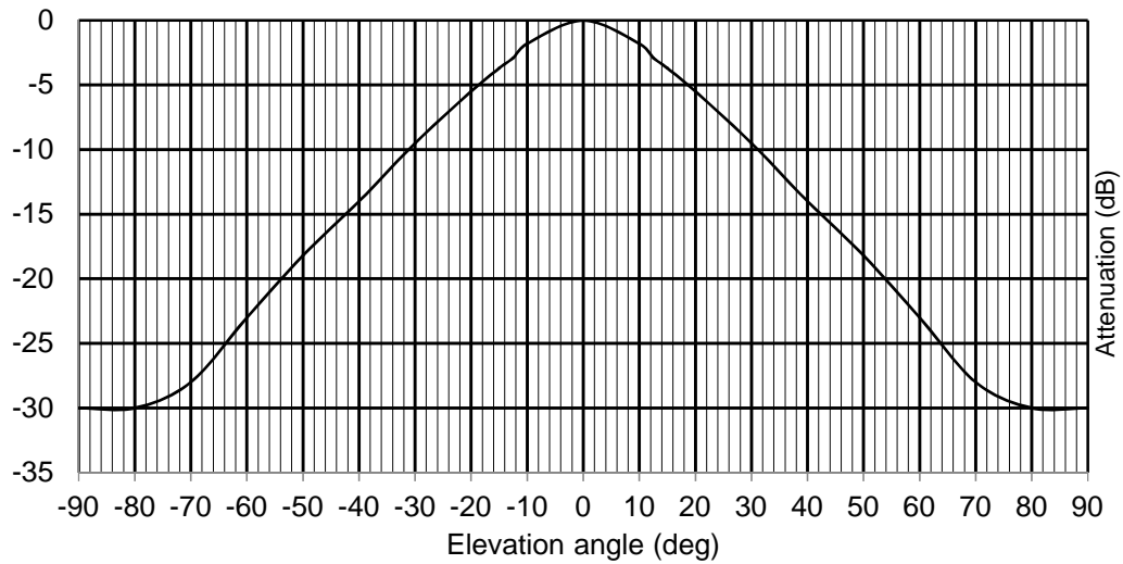
Figure 4: Minimum attenuation of the vertical antenna pattern
