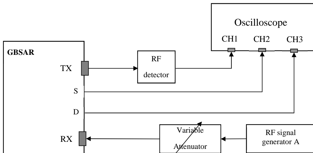
Figure 8: DAA measurement arrangement
