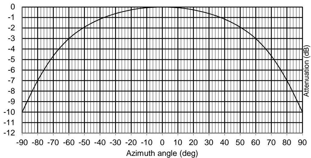
Figure 5: Minimum attenuation of the horizontal antenna pattern
