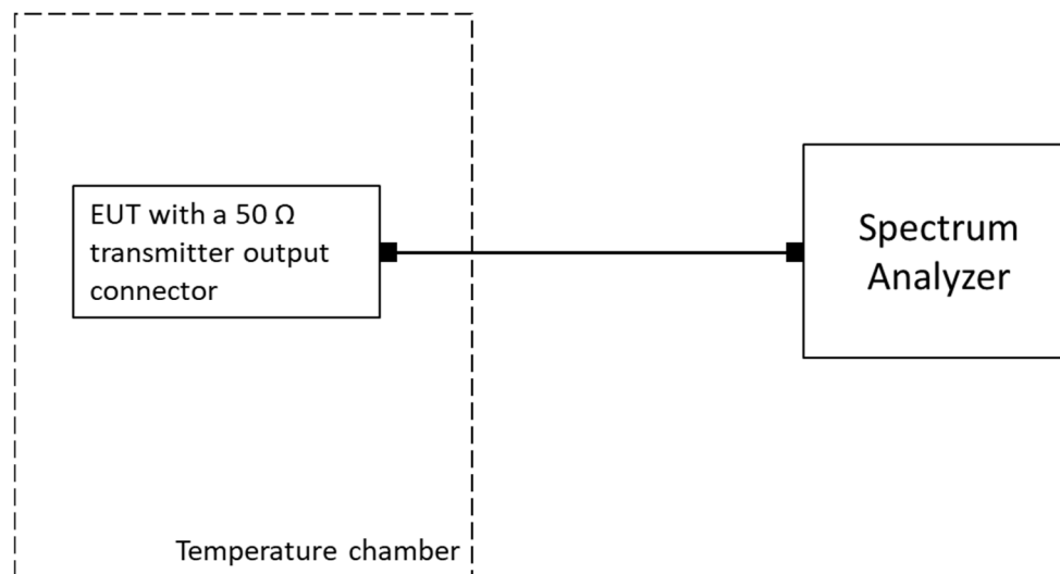
Figure 6: Setup for conducted measurements
